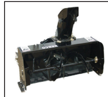
Snow Blower - Two Stage, hydraulically driven, with discharge spout adjustable for distance and direction. 40" or 60" widths.
