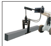
Curb Mover - Clamps and standard concrete parking curbs, 40' long boom, hydraulically.
