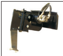
Vibratory Plow-Compactor Pull pipe or cable to 12" deep in difficult soil with minimum surface disturbance. 8" by 10" rectangular compactor shoe compacts sub-bases.
