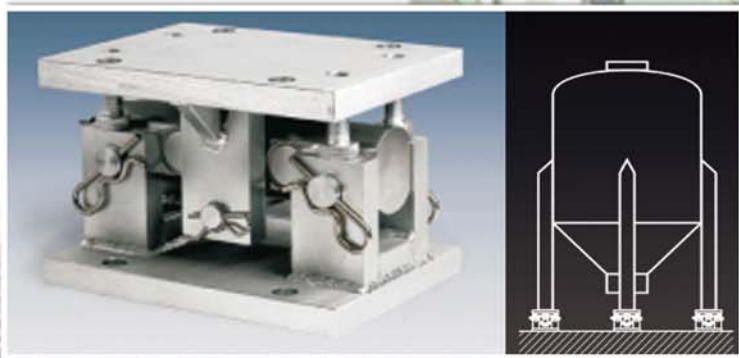
load cell weighing system
